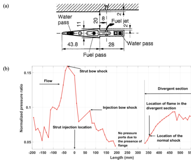
Fig 1. (a) Strut design for the combustor, (b) Pressure distribution along the combustor
